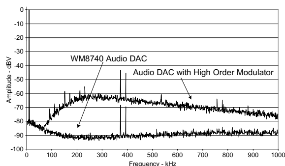
Figure 10. Out-of-band DAC spectra (from [17]).
