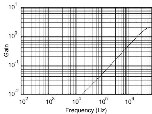
Figure 6. Period jitter implicit filter.
