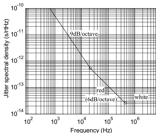
Figure 3. Asymptotes of oscillator jitter spectra.
