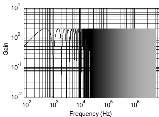
Figure 7. 1ms interval jitter implicit filter.
