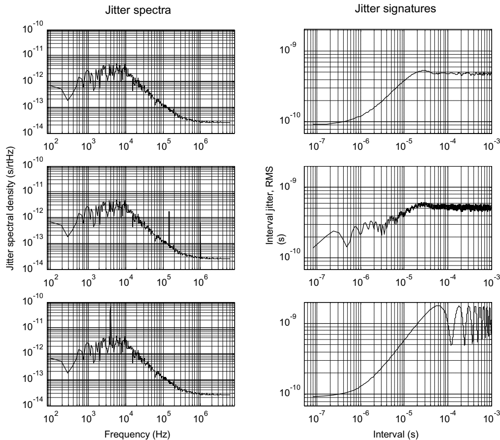
Figure 8. Jitter spectra/signature pairs.
