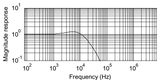
Figure 9. PLL jitter transfer function.
