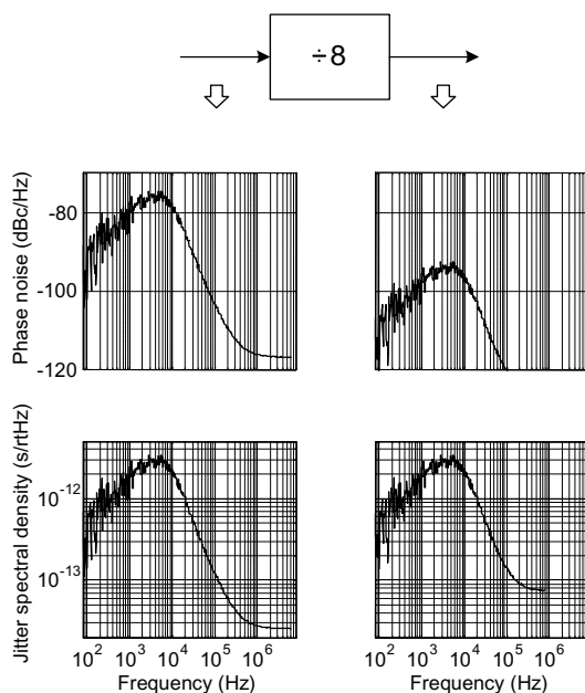
Figure 11. The effect of clock division.
