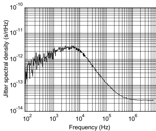
Figure 4. Idealized PLL jitter spectrum.
