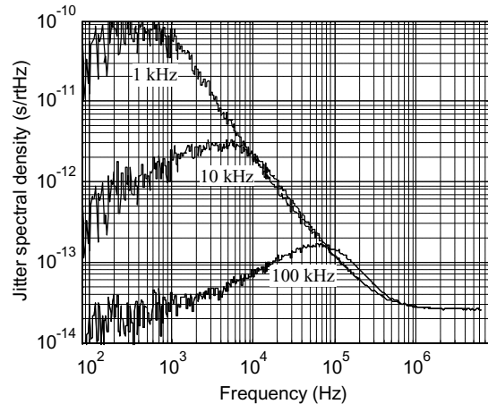
Figure 5. Spectra for different PLL bandwidths.
